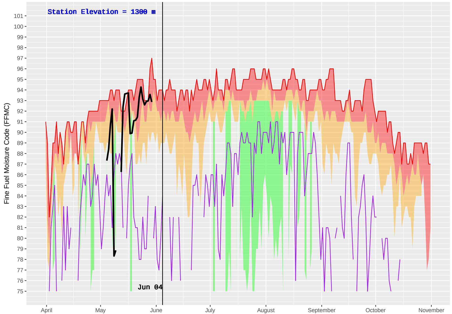
MARION (367) : Historical (1994–2016) and Current (2018) Noon Fine Fuel Moisture Code (FFMC)
